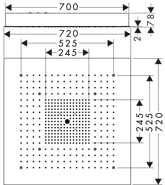
Scale drawing
