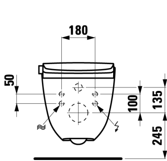
Connection with Laufen installation system LIS CW2
