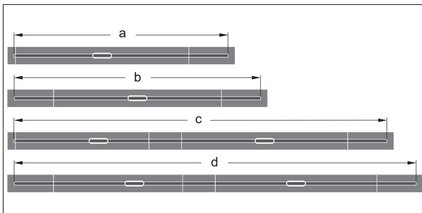
Fig. 1: Installation possibilities with end closing piece
