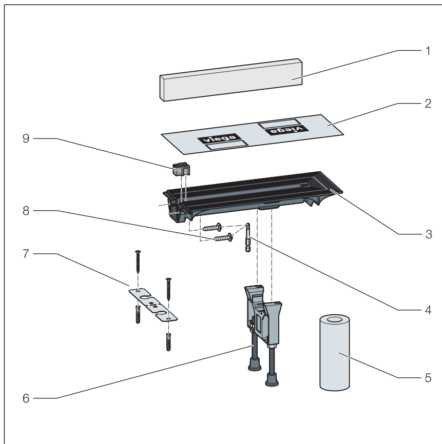
Fig. 2: end closing piece, scope of delivery
