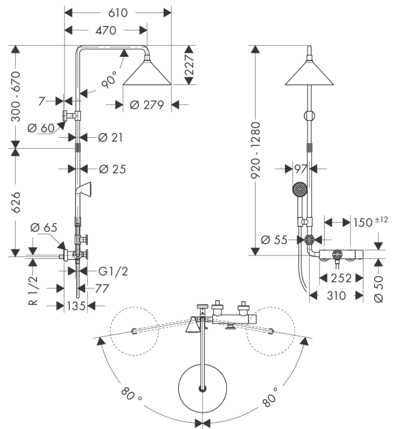
Scale drawing
