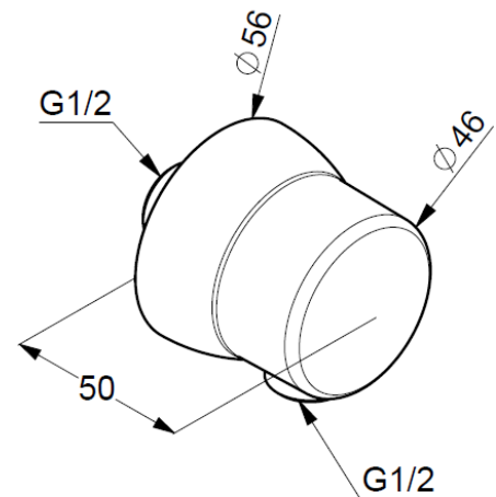
Dimensional drawing
