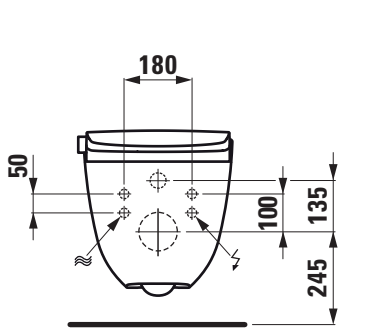
Connection with Laufen installation system LIS CW2
