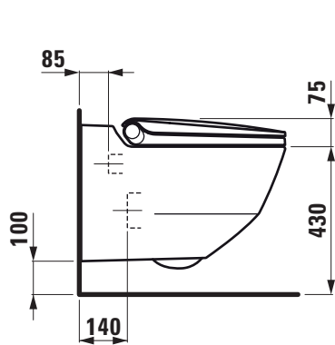
Connection with commercially available installation systems
